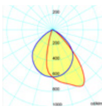
QUASAR 30 LED Bred ned
