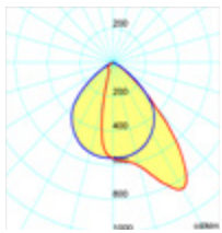
QUASAR 20 LED Bred ned
